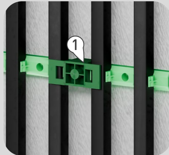
1. Fastening element with dowel (art. no. 4050000013) 8 pieces per m 2 active area
