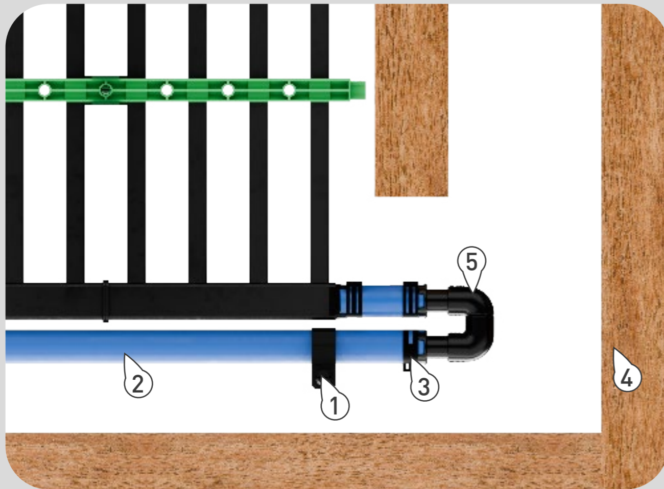
Detail: Connection
