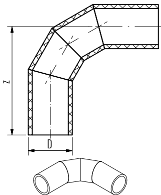
pipe segments
