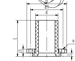
socket welding
