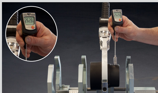
Temperature control aquatherm welding machine
