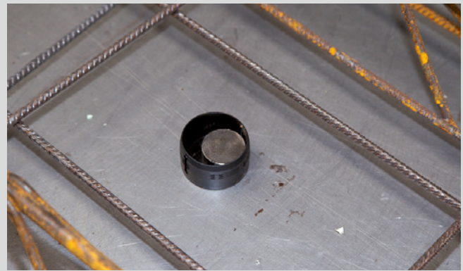
Base part of sprinkler outlet Art. no. 3090000001 for visible sprinklers. Attachment by magnet.
